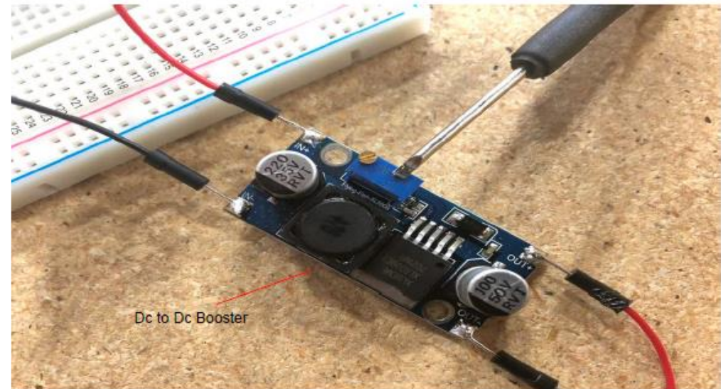
Measure voltage first, before adding to circuit. Have 12vdc to IN+ and IN- and measure OUT+ and OUT- for 18 to 24vdc (no higher) by adjusting the blue potentiometer.
